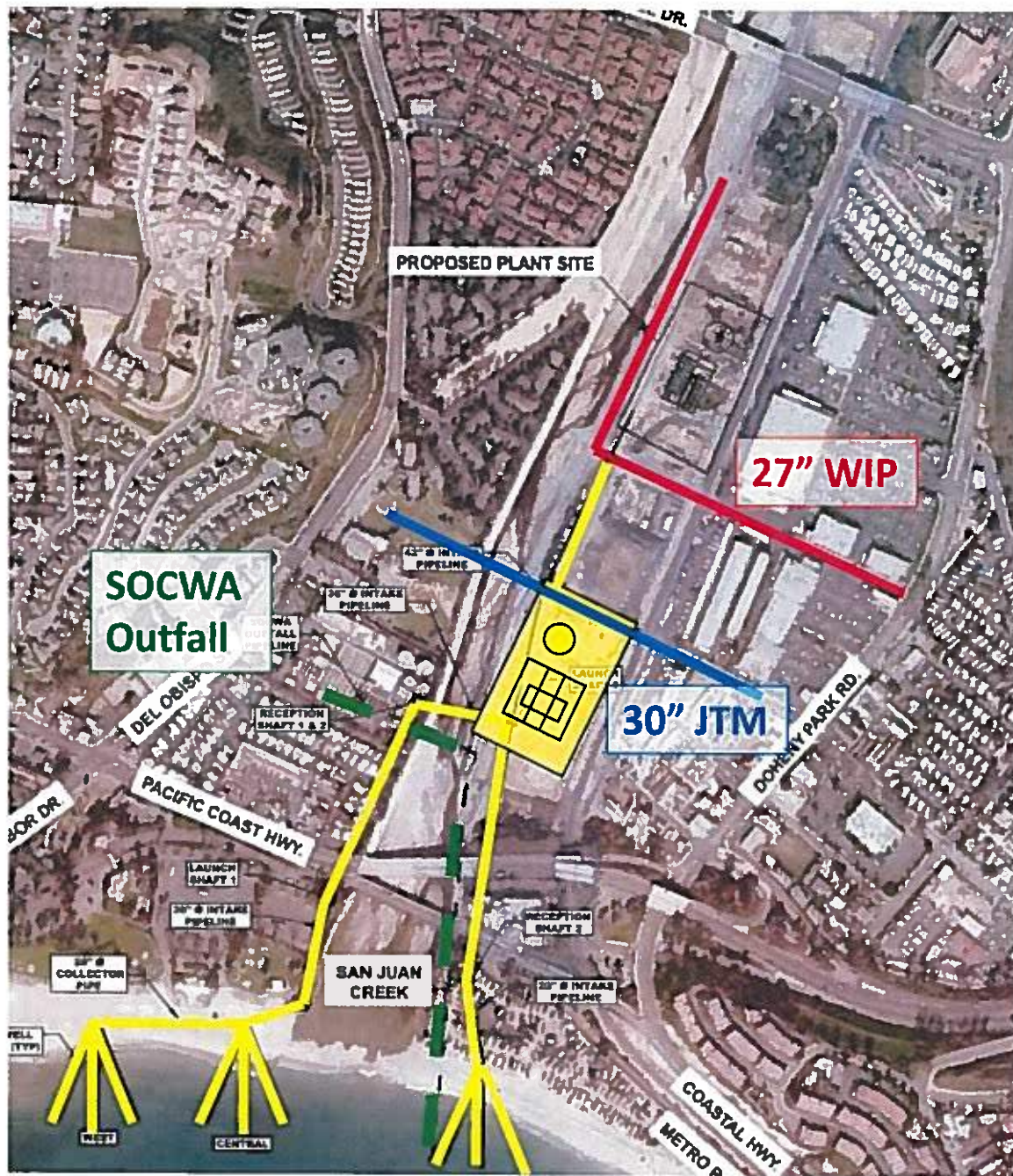
Figure 1B - Schematic of Doheny Desal Project Layout
