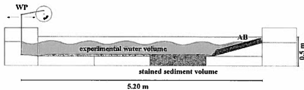
Fig. 1. The laboratory wave tank (light gray, scaled off water volume; dark gray, experimental water volume; WP, wave paddle; AB, artificial beach).
