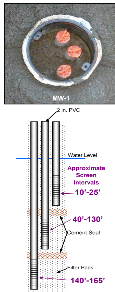
Figure 2-2. General Monitoring Well Construction
