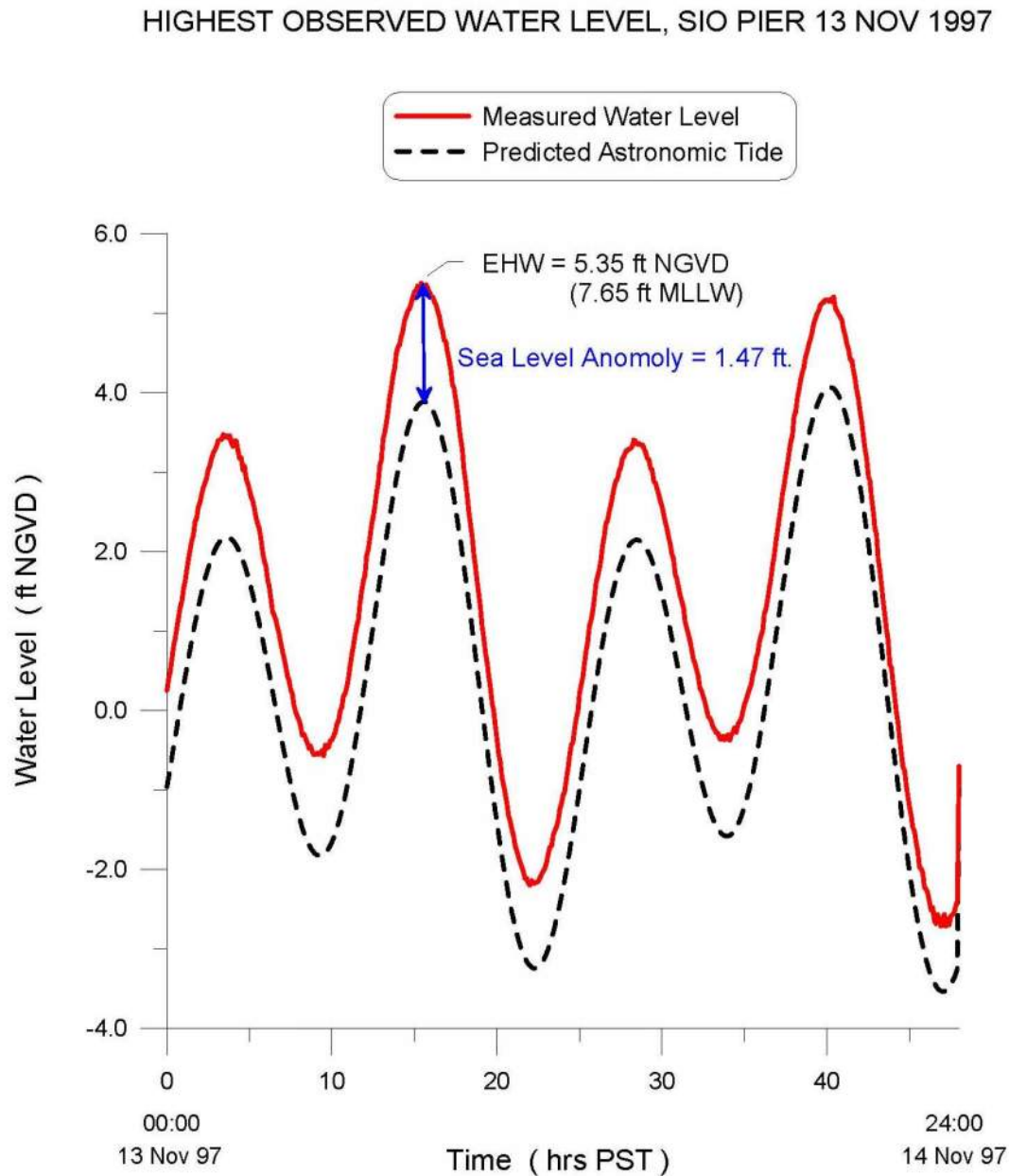
Figure 4.2: Comparison of measured ocean water level (red) at the Scripps Pier tide gage vs. predicted water level based on tidal constituents (black dashed) for the extreme high water event of 13 November 1997 (from Jenkins and Wasyl, 2005).
