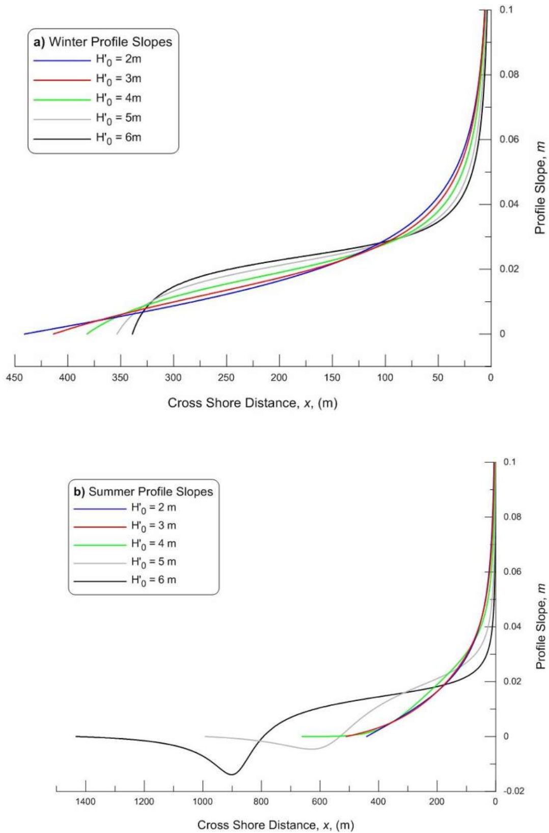
Figure 6.12. Family of elliptic cycloid slope solutions in the bar berm: a) type-a cycloids; b) type-b cycloids. Cycloids scaled for : H'_0 = 2 - 6\text{ m} ; T = 15\text{ sec} ; m_{DIM} = 0.06 (winter); m_{DIM} = 0.1 (summer); \gamma = 0.8 ; \Gamma = 0.76 ; \Lambda = 0.81
