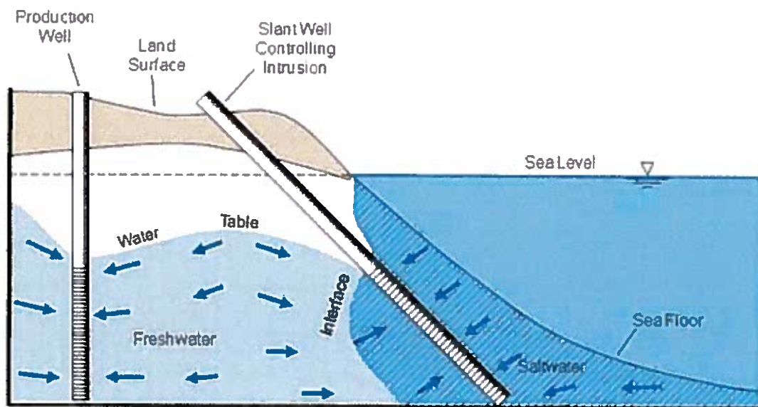
Figure 10. Slant Wells Intercepting Seawater Providing Seawater Intrusion Control
