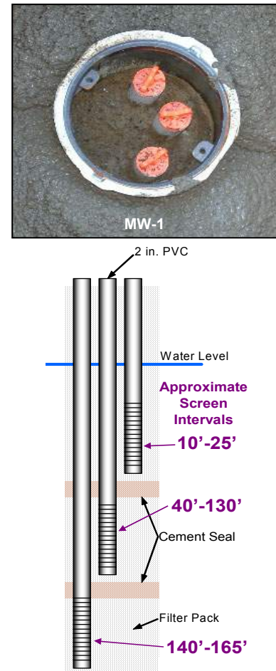
Figure 6. General Monitoring Well Construction
