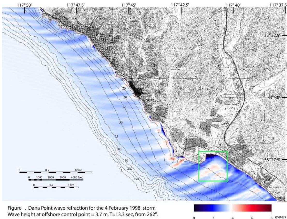
Figure 6.6: Wave refraction/diffraction field around the SJCOO site and the Doheny Desalination Project site derived from wave burst measurements from the Acoustic Doppler Current Profiler (ADCP) records taken under the MBC Applied Environmental Sciences (MBC) NPDES monitoring studies. Nearfield domain of the SJCOO and the Doheny Desalination Project site designated by green box.
