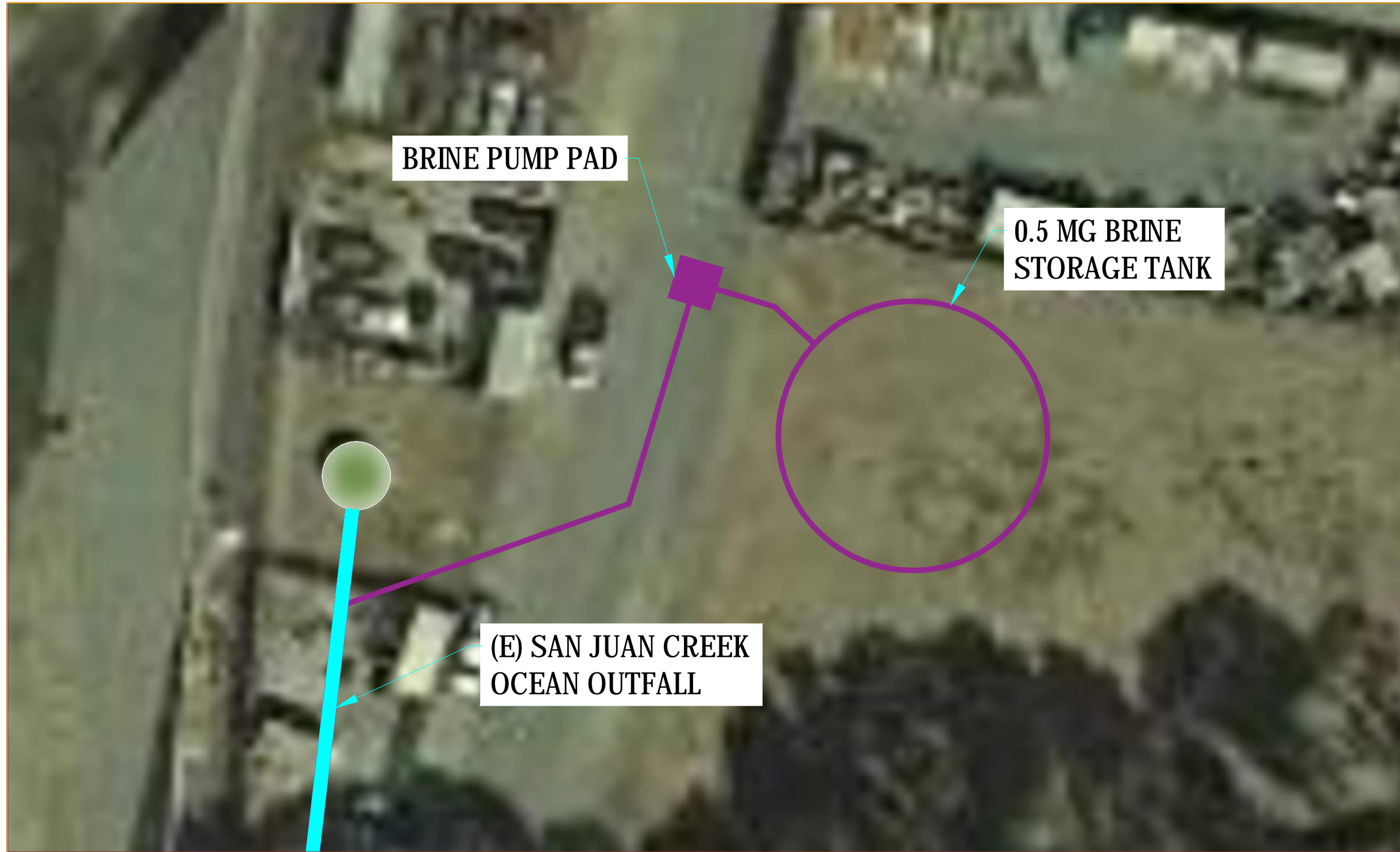
2 BRINE STORAGE TANK - CONNECTION TO SAN JUAN CREEK OCEAN OUTFALL 1" = 25'
