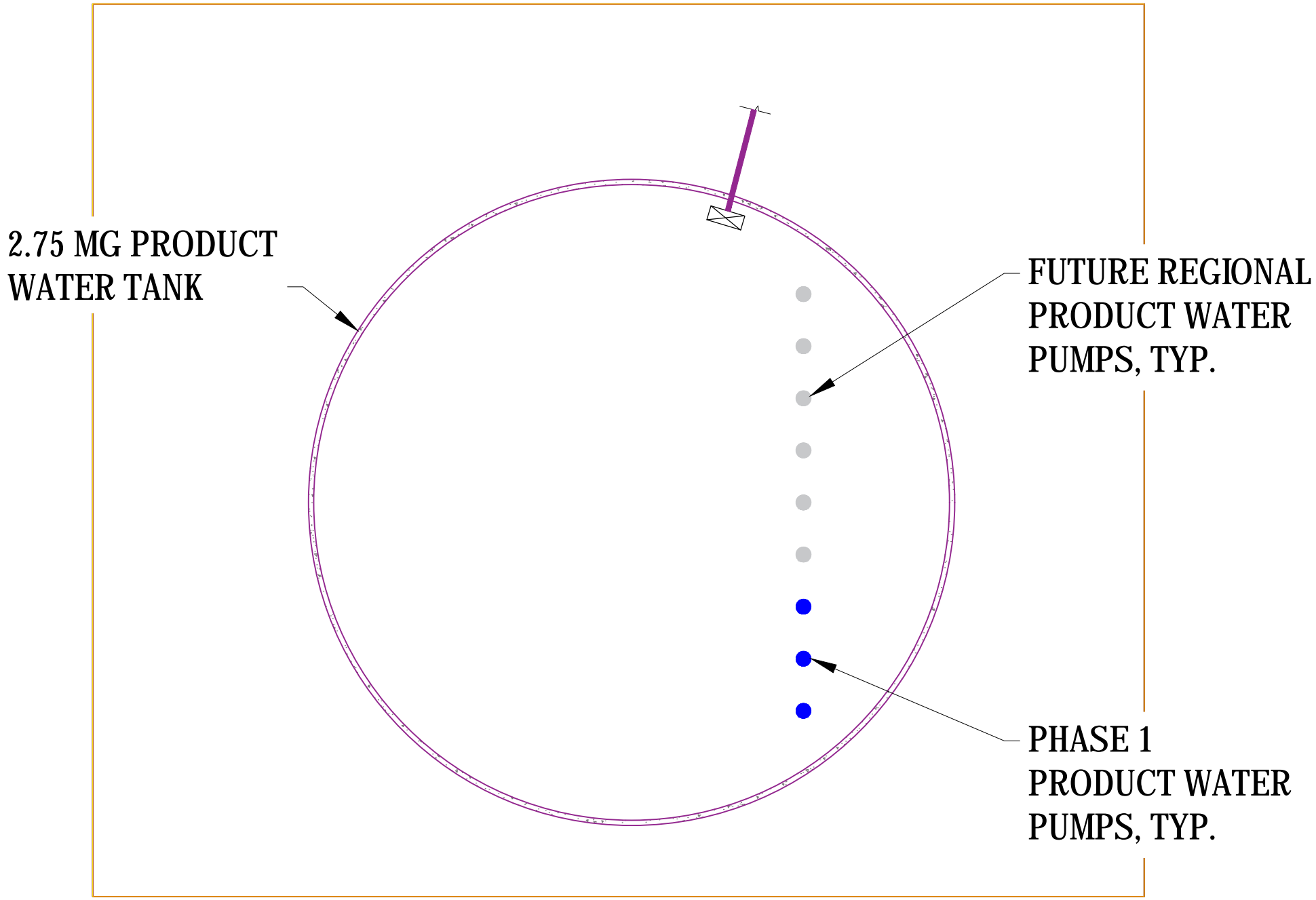
1 PRODUCT WATER STORAGE TANK AND PUMPS 1" = 25'
