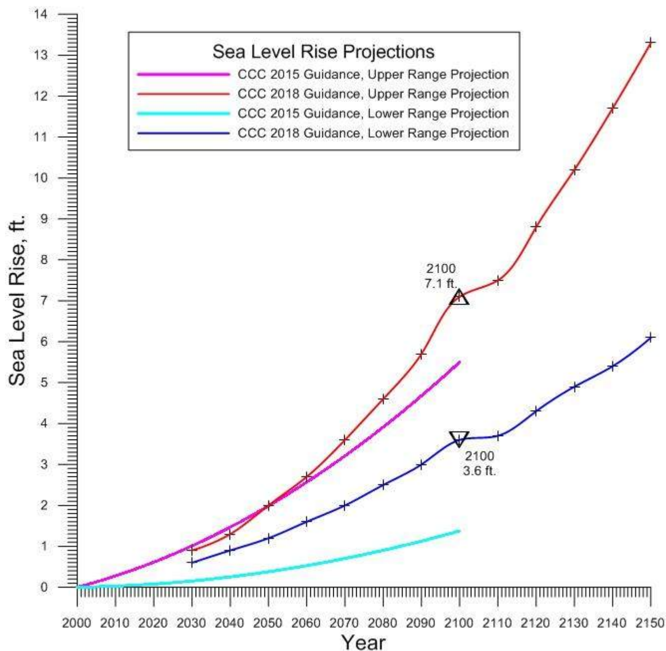
Figure 3.1: Range of sea level rise projections from the California Coastal Commission sea level rise guidance document, (CCC, 2018, Appendix-G). The 2100 planning horizon is indicated by symbols on the upper and lower range curves. Blue curve represents a 17% probability that sea level rise exceeds these values; red curve represents a 0.5% probability that sea level rise exceeds these values
