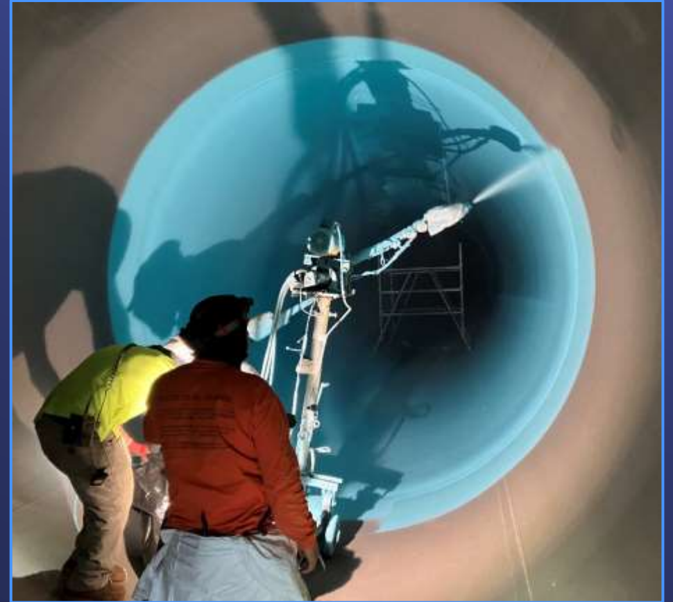
Contractor applying polyurethane liner to interior of pipe
