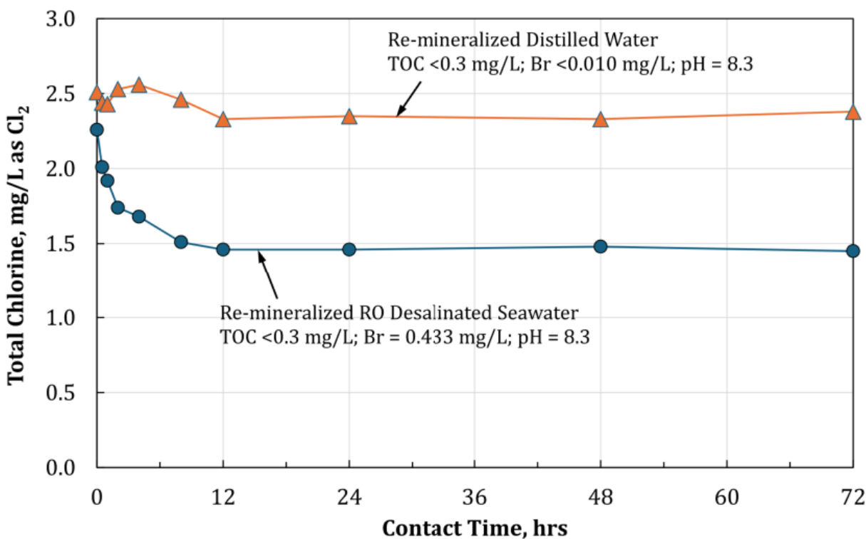
Figure 5.2 Impact of Bromide on the Decay of Total Chlorine in Buffered TOC-Free Water
