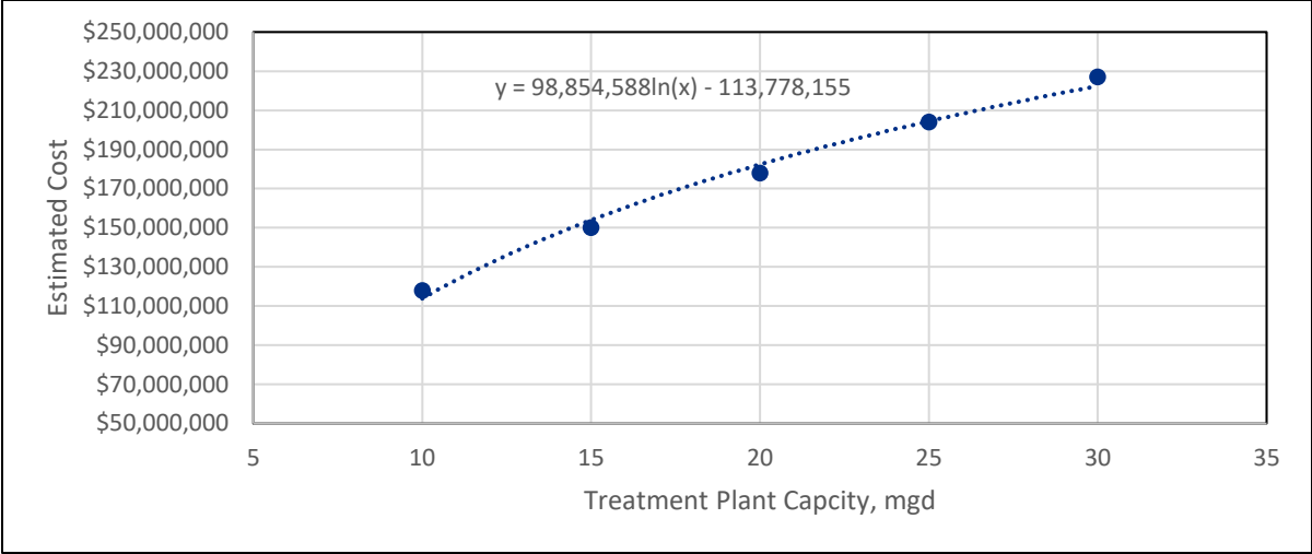
Figure 7.6 Treatment Process Cost Factor Curve
