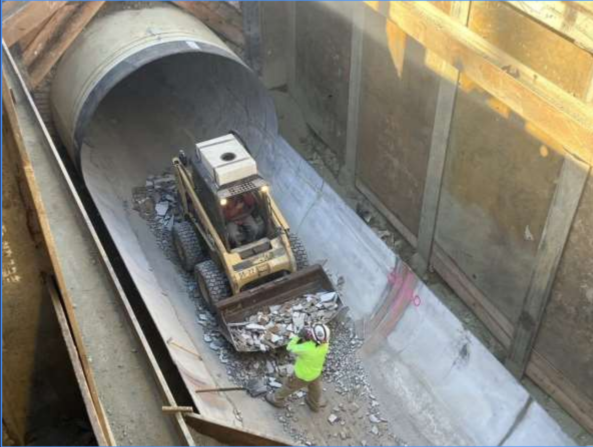
Removal of damaged cement mortar lining
